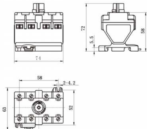
CZ0201 板前导轨型防爆 H 四极开关模块 Board front mounting rail type explosion-proof H 4-Pole switch module
