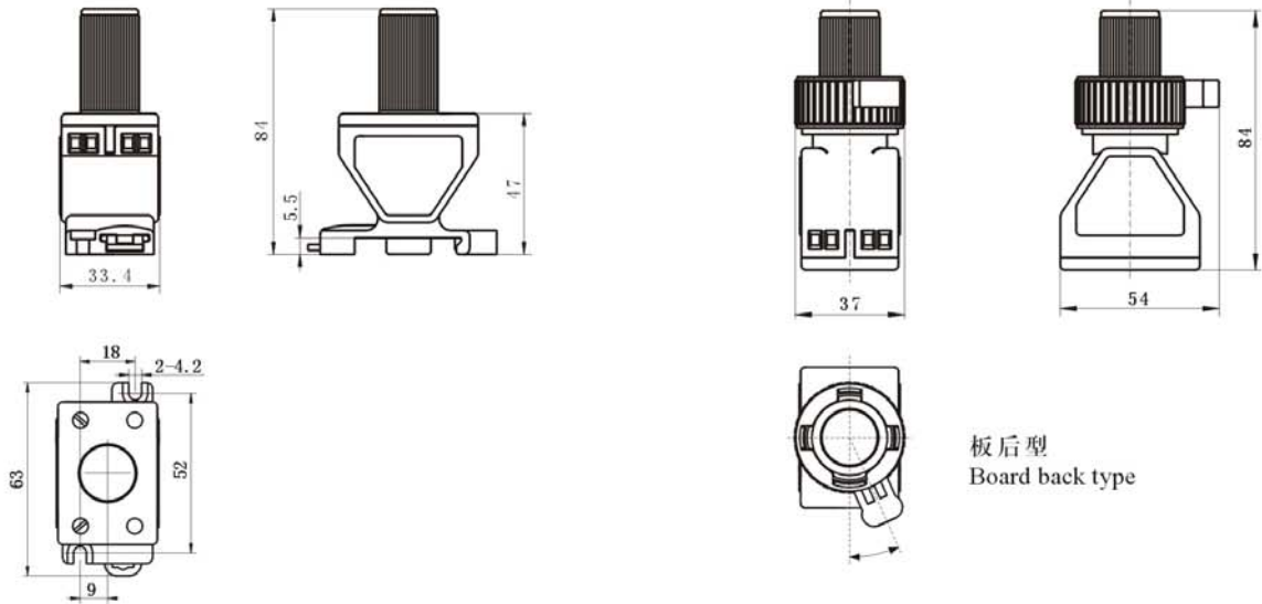
板前导轨型 Board front mounting rail type
