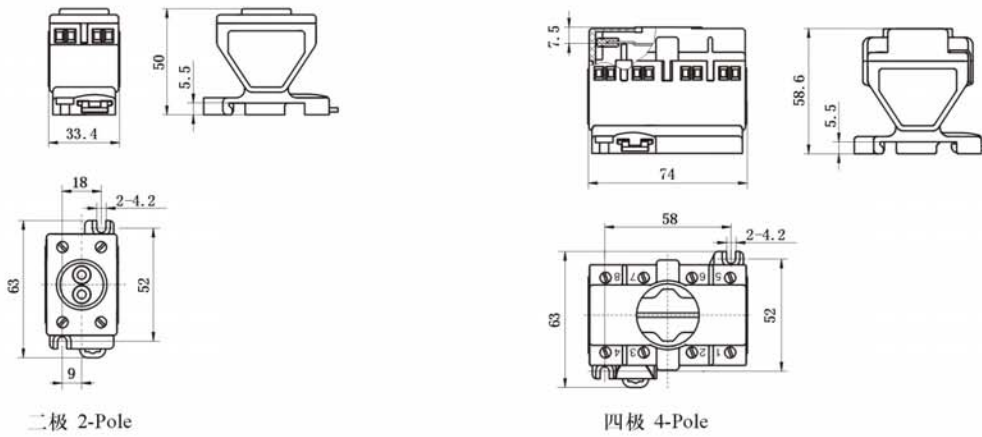
CZ0201 板前导轨型防爆开关模块 Broad front mounting rail type explosion-proof switch module
