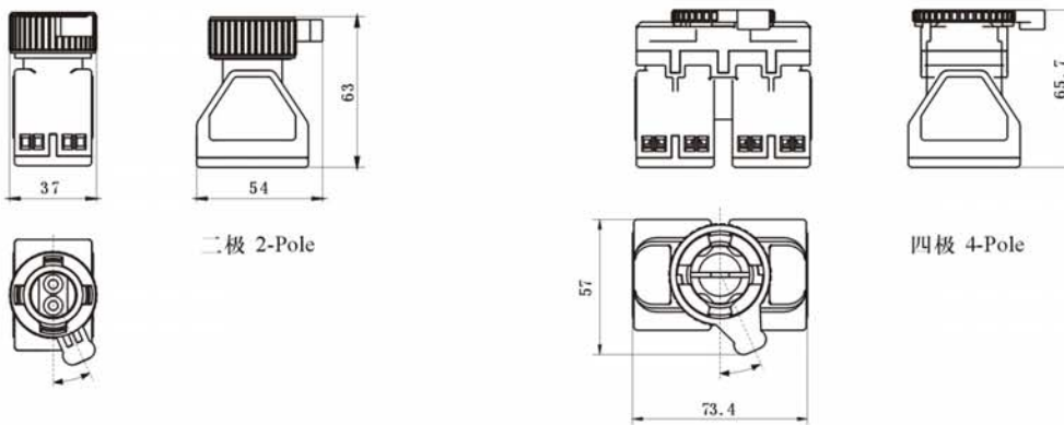
CZ0201 板后型防爆开关模块 Board back type explosion-proof switch module
