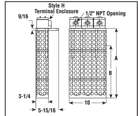
QM3 — Dimensions (Inches)
