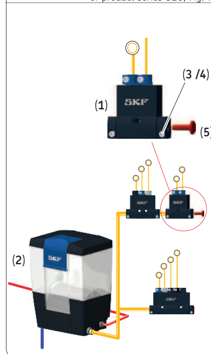
Single-line system with lubricant distributors of product series 310, Fig. 7
