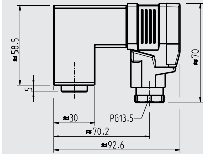
with angular connector form A and flange connection
