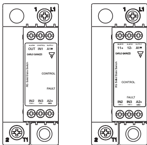
RGC...D9xGGEP RGC...A9xGGEP
